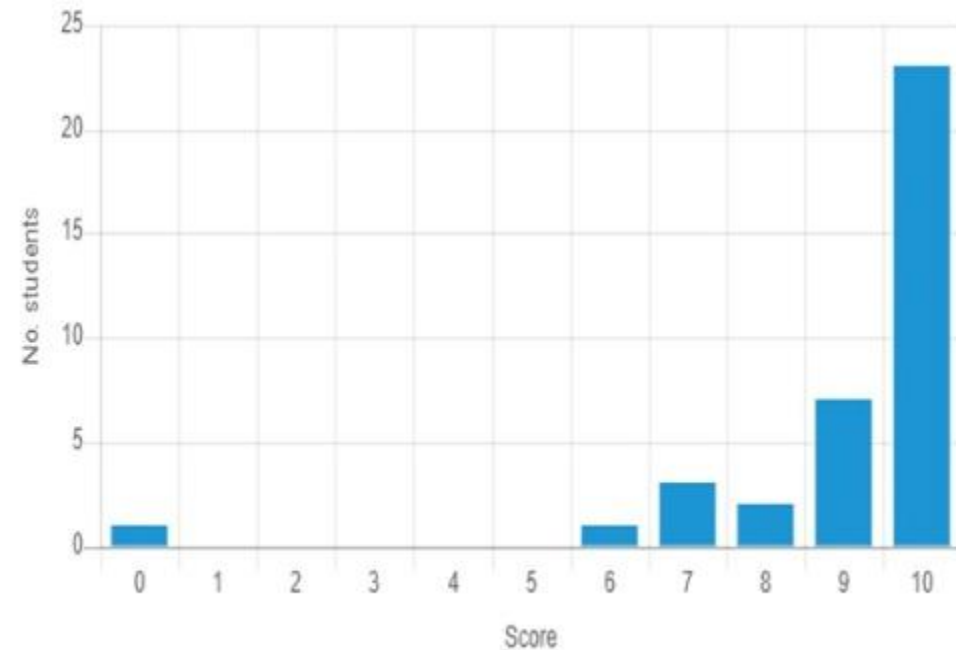
Score distribution
